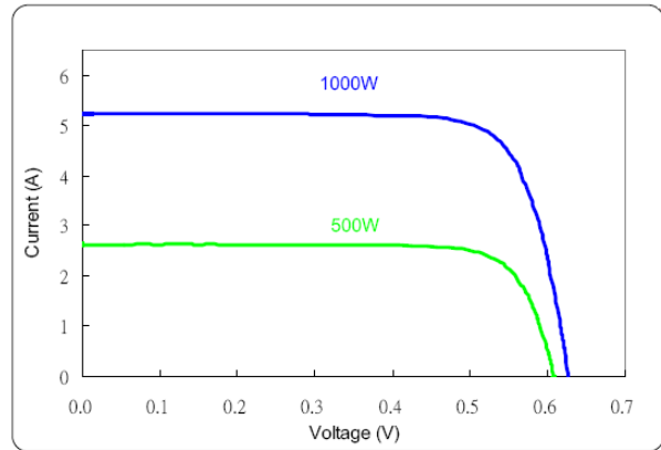
IV-CURVE OF CELL (EFFICIENCY =17.2%) :
